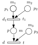
Fig. 5. Two places to two places model
