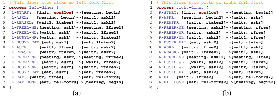
Fig. 1. Behavioral Automata for (a) “Left” Philosophers (b) “Right” Philosophers
