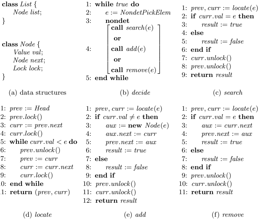
Fig. 1. Data structure and algorithms for concurrent lock-coupling list
