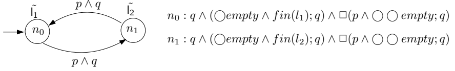
Fig. 4. LNFG of q \wedge (\bigcirc \text{empty}; q) \wedge \Box(p \wedge \bigcirc \bigcirc \text{empty}; q)
