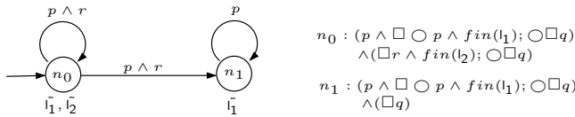
Fig. 3. LNFG of (p \wedge \square \bigcirc p; \bigcirc \square q) \wedge (\square r; \bigcirc \square q)
