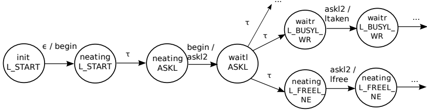
Fig. 3. Part of 1E_l
