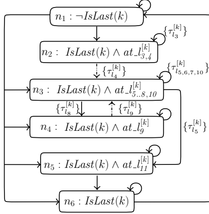
Fig. 8. Verification diagram \Psi for \|_{j < N} T_j \models \psi(k)
