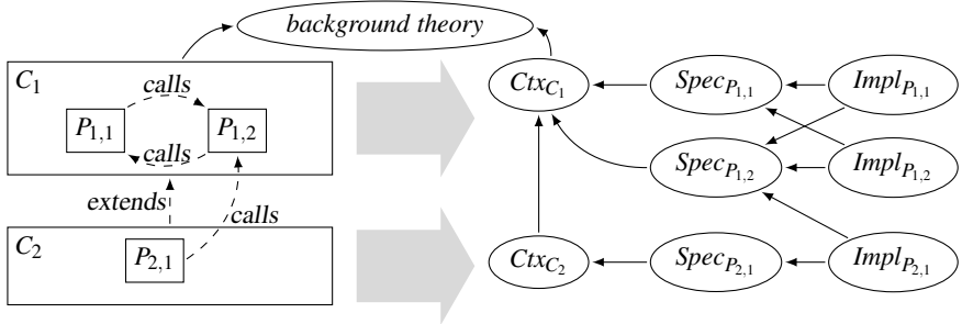
Fig. 2. Example PVS translation of two contexts. Contexts and procedures are drawn as boxes, theories as ellipses, calls and extends relations as dashed arrows, and importing relations as continuous arrows.
