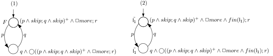
Fig. 5. LNFG of (p \wedge \text{skip}; q \wedge \text{skip})^+ \wedge \Box \text{more}; r
