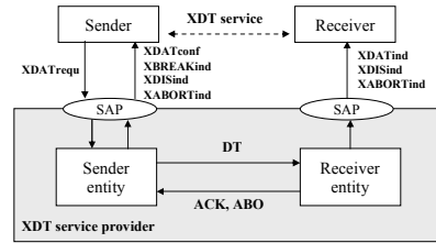
Fig. 8. XDT service and protocol
