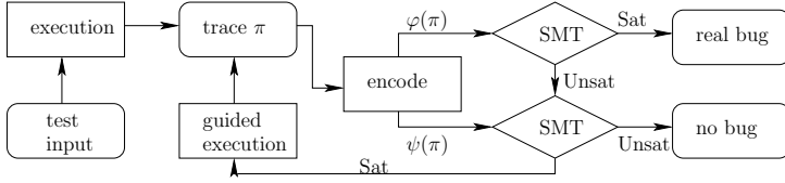
Fig. 2. Trace-driven verification flow
