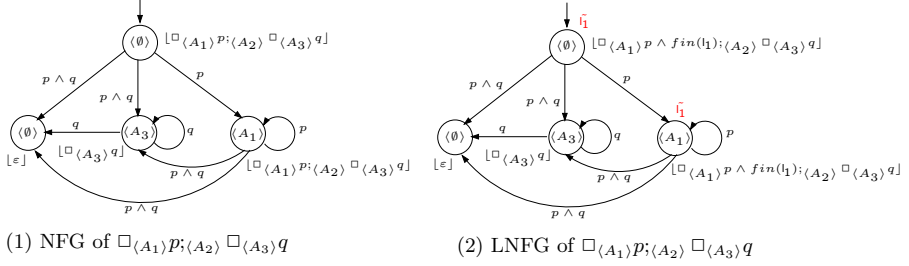
Fig. 5. NFG and LNFG of \Box_{\langle A_1 \rangle} p; \langle A_2 \rangle \Box_{\langle A_3 \rangle} q
