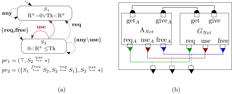
Fig. 4. (a) Top-level requirement \varphi ; (b) Composition \mathcal{I}_{\text{Net}} for contract \mathcal{C}_{\text{Net}}
